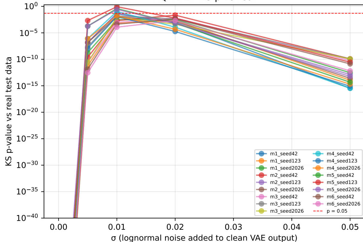
RQA-DET KS p vs real
