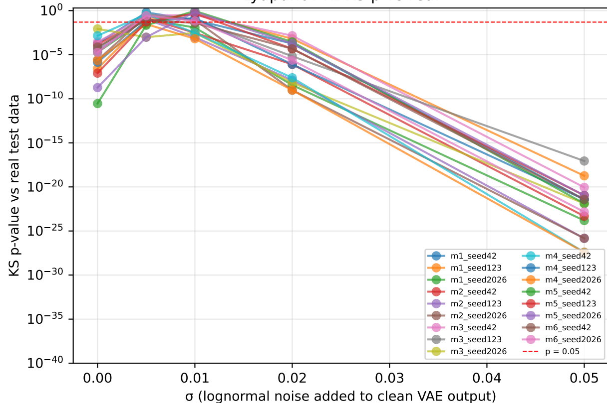
Lyapunov \lambda_1 KS p vs real
